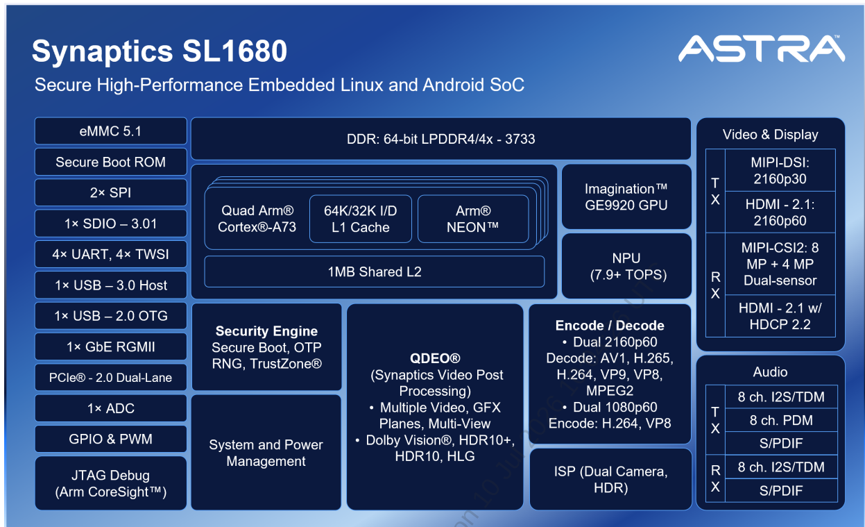
Figure 1. Astra SL1680 High-level block diagram
