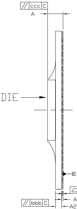
Figure 20. SL1680 Side View
